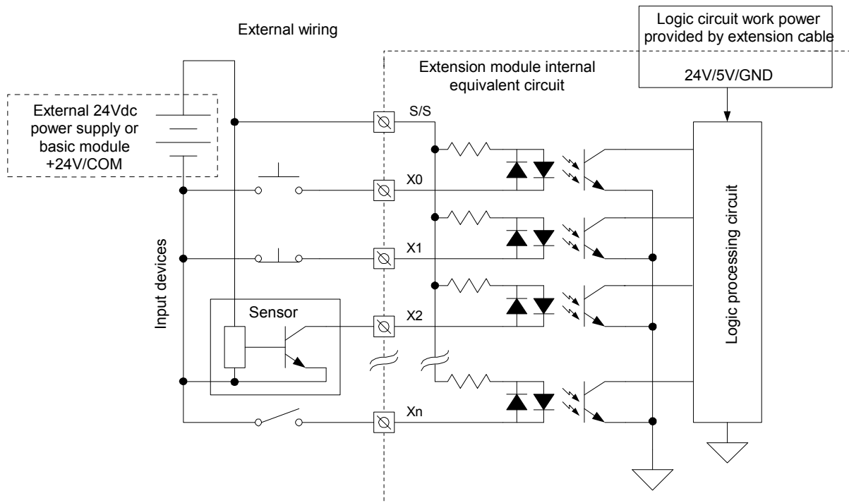
Figure 4-16 I/O extension module internal equivalent input circuit
