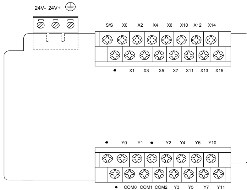
Figure 4-8 Terminals of IVC1-1410MDR and IVC1-1410MDT
