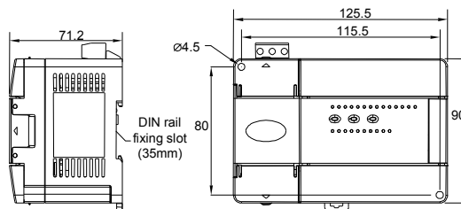
Figure 6-1 Cutout sizes of IVC1-1006MAR and IVC1-1006MAT, IVC1-1006MDR and IVC1-1006MDT
