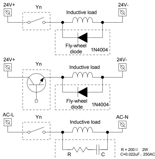
Figure 4-25 Protection circuit of PLC output contact
