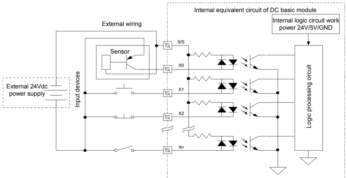
Figure 4-15 Source input mode internal equivalent circuit of DC basic module
