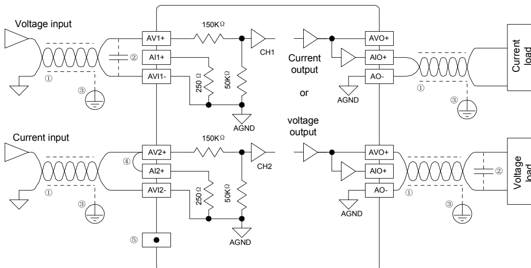
Figure 4-29 Internal equivalent circuit of analog I/O
