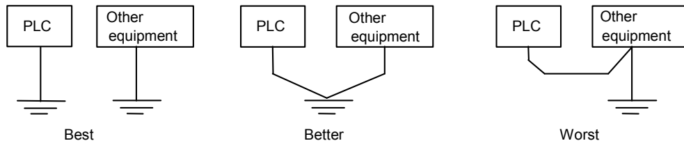
Figure 6-12 PLC grounding method
