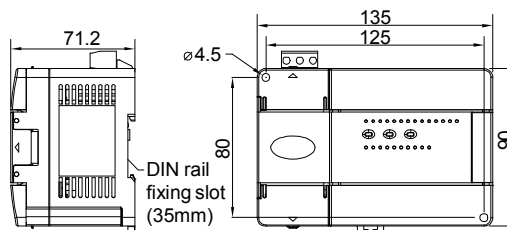
Figure 6-2 Cutout sizes of IVC1-1410MAR, IVC1-1410MAT, IVC1-1410MDR and IVC1-1410MDT
