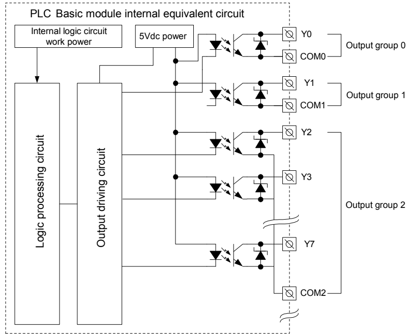
Figure 4-26 Output terminal internal equivalent circuit of transistor output type PLC
