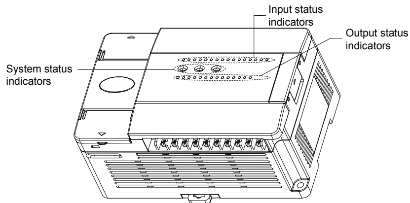
Figure 4-28 Basic module status indicator position
