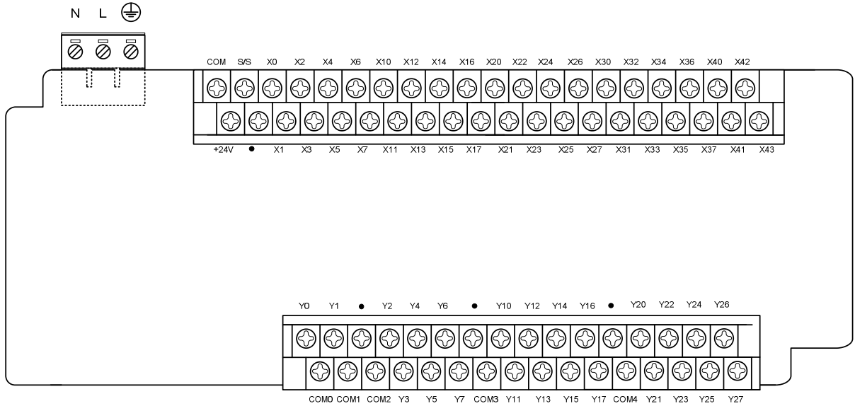
Figure 4-5 Terminals of IVC1-3624MAR and IVC1-3624MAT
