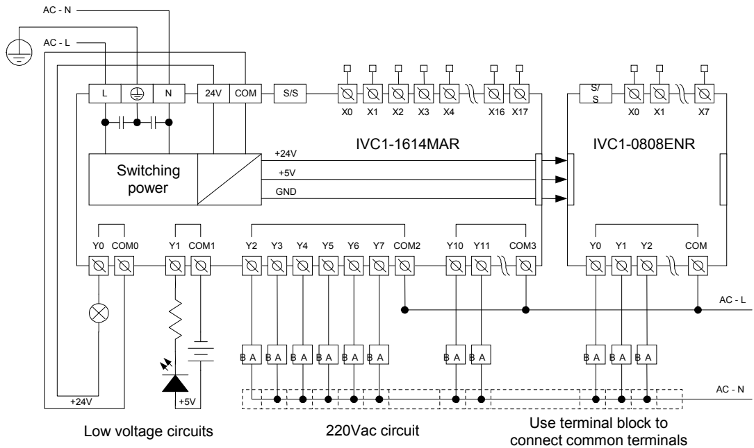
Figure 4-27 Electric connection between IVC1-1614MAR and IVC1-0808ENR
