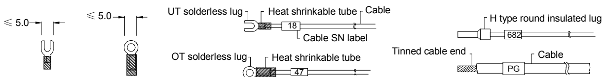
Figure 6-10 PLC cable processing method
