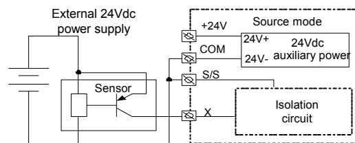
Figure 4-18 Wiring of source input mode using external auxiliary power
