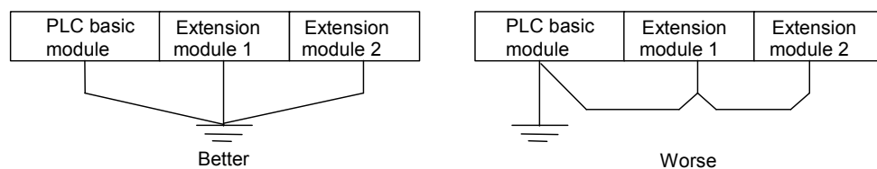
Figure 6-13 Grounding of PLC basic module and extension modules
