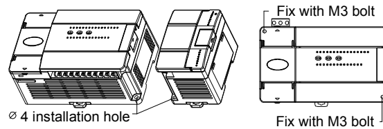
Figure 6-9 Screw fixing
