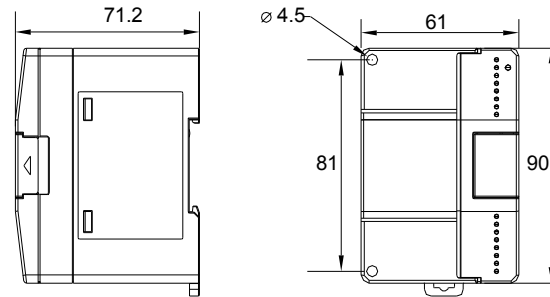
Figure 6-6 Cutout sizes of I/O extension module and special function module
