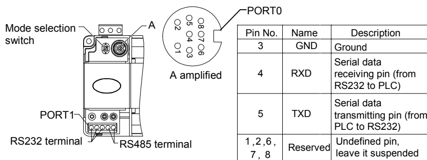
Figure 5-1 Communication port and mode selection switch
