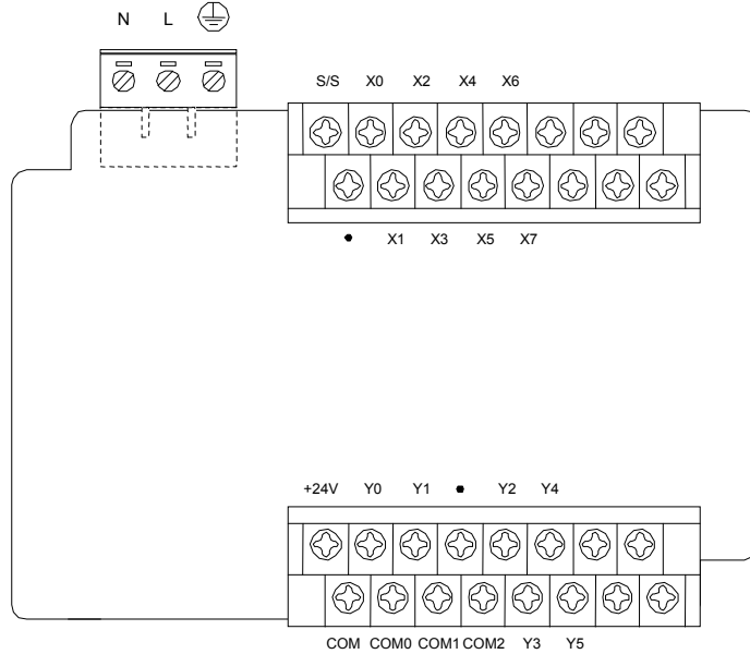
Figure 4-1 Terminals of IVC1-1006MAR and IVC1-1006MAT
