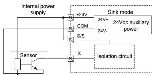
Figure 4-19 Wiring of sink input mode using module internal power
