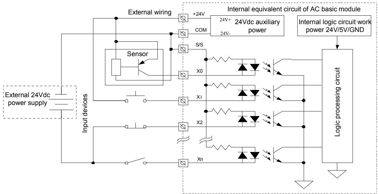
Figure 4-14 Source input mode internal equivalent circuit of AC basic module
