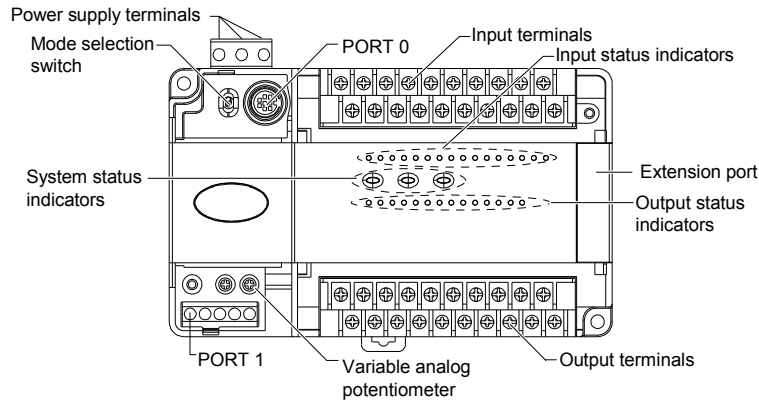
Figure 2-1 Structure of IVC1 series basic module (take IVC1-1614BRA as an example)
