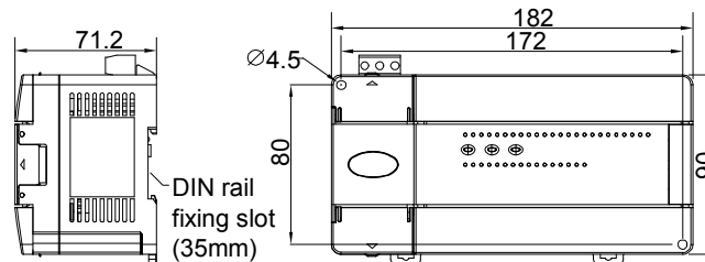
Figure 6-4 Cutout sizes of IVC1-2416MAR, IVC1-2416MAT, IVC1-2416MDR, IVC1-2416MDT, IVC1-1614MAR1 and IVC1-1614MAT1
