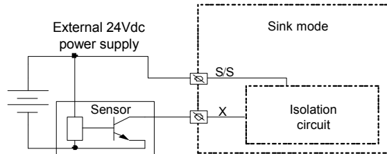
Figure 4-22 Wiring of sink input mode for DC basic module
