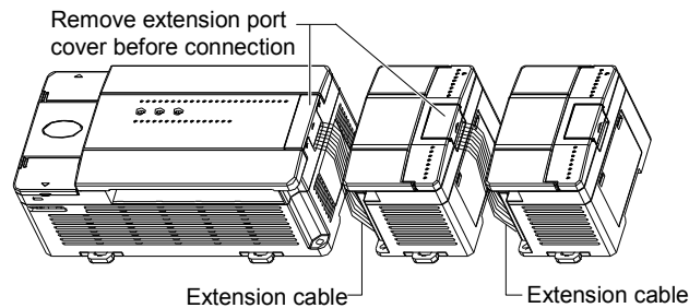
Figure 6-14 Connecting extension module
