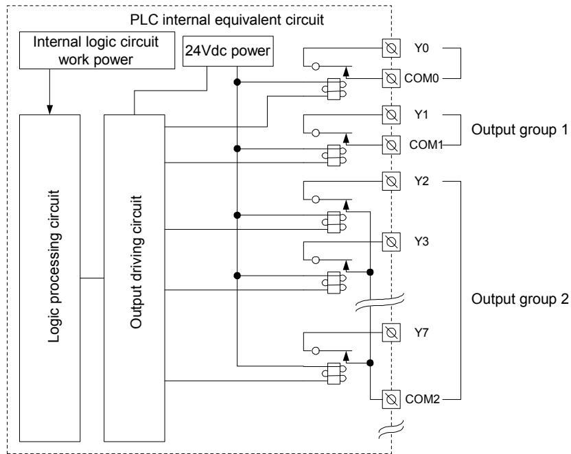
Figure 4-24 Output terminal internal equivalent circuit of relay output type PLC
