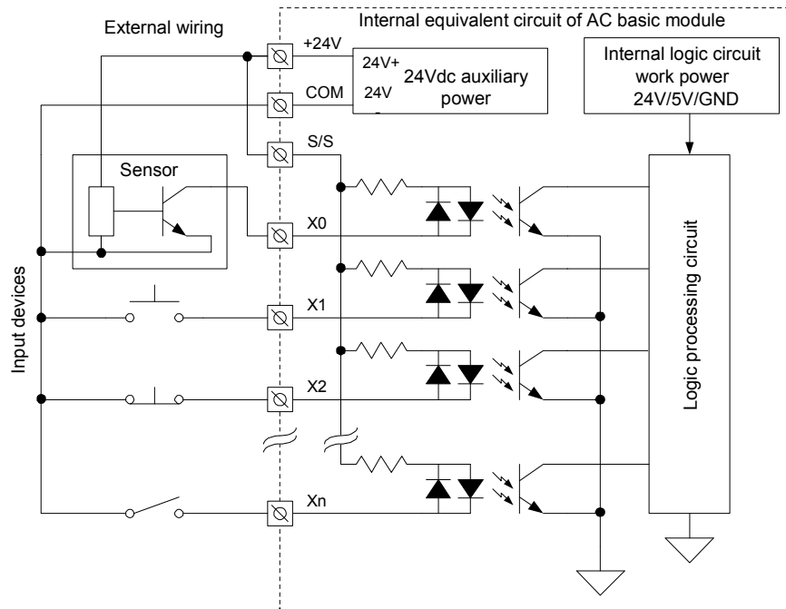
Figure 4-12 Sink input mode internal equivalent circuit of AC basic module
