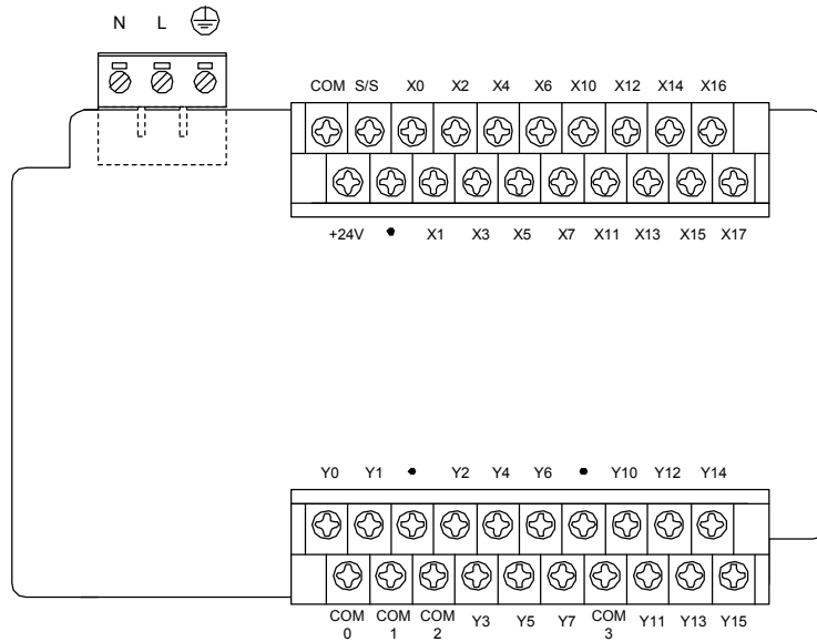
Figure 4-3 Terminals of IVC1-1614MAR and IVC1-1614MAT
