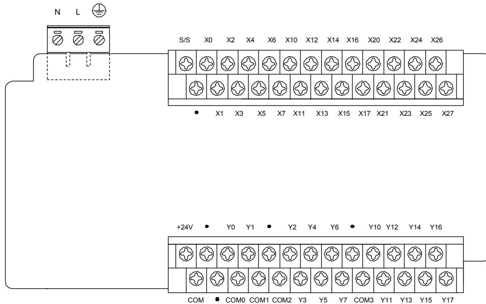
Figure 4-4 Terminals of IVC1-2416MAR and IVC1-2416MAT
