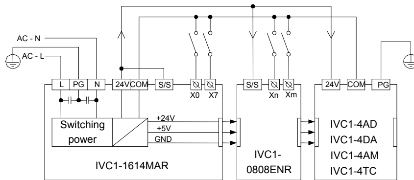
Figure 6-11 Connecting AC power and auxiliary power
