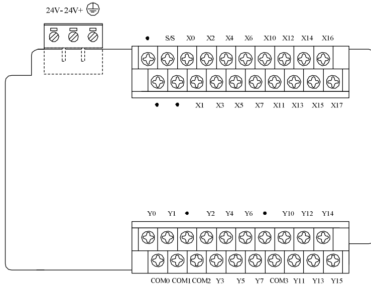
Figure 4-9 Terminals of IVC1-1614MDR and IVC1-1614MDT
