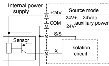
Figure 4-17 Wiring of source input mode using module internal power
