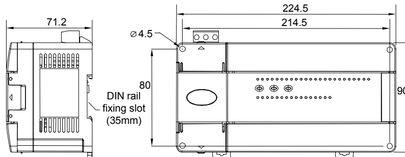
Figure 6-5 Cutout sizes of IVC1-3624MAR, IVC1-3624MAT, IVC1-3624MDR and IVC1-3624MDT
