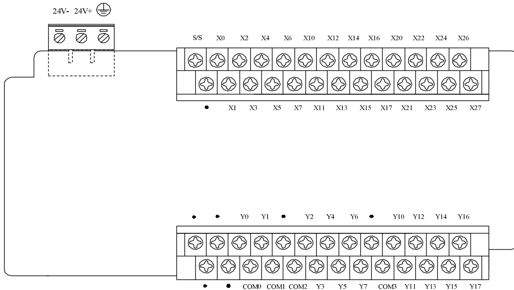
Figure 4-10 Terminals of IVC1-2416MDR and IVC1-2416MDT
