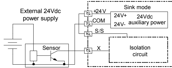
Figure 4-20 Wiring of sink input mode using external auxiliary power
