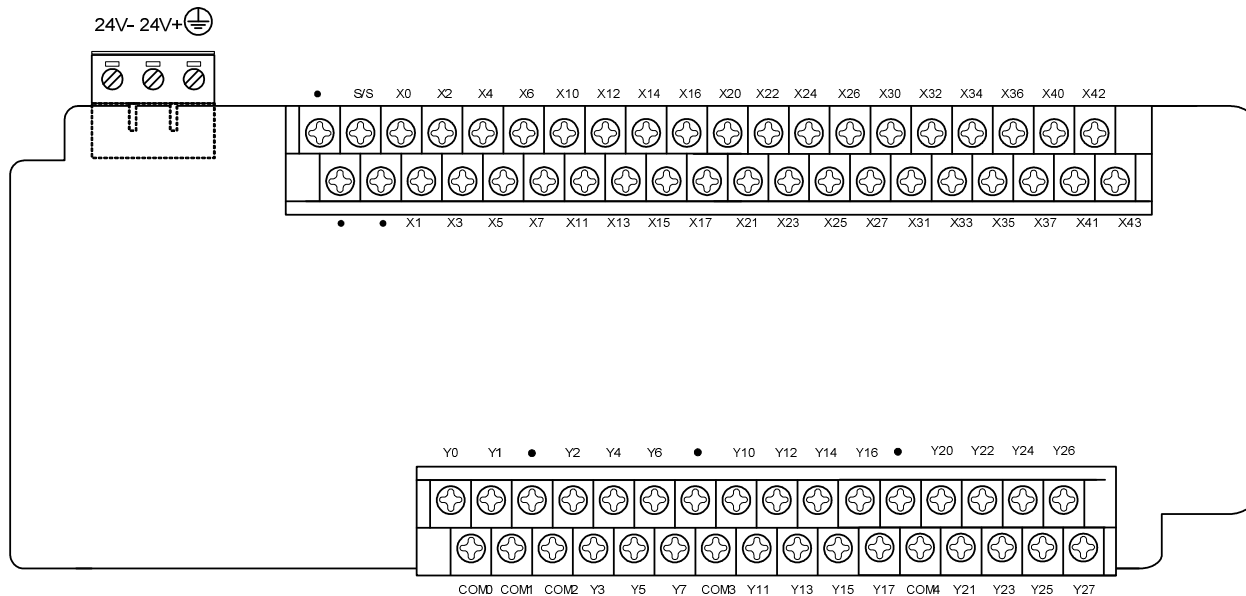
Figure 4-11 Terminals of IVC1-3624MDR and IVC1-3624MDT
