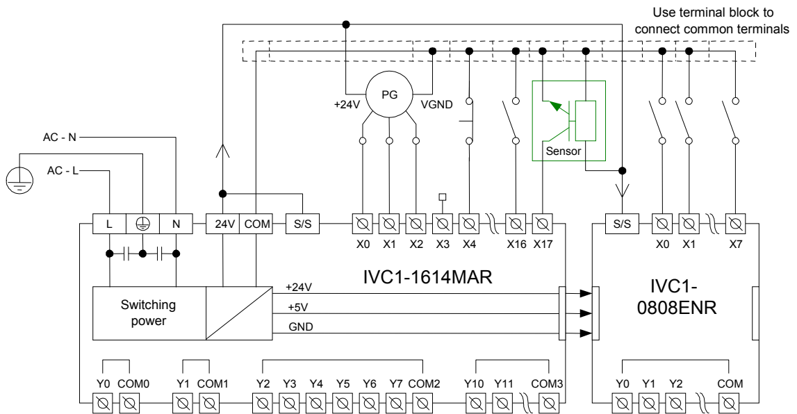
Figure 4-23 Electric connection of IVC1-1614MAR and IVC1-0808ENR
