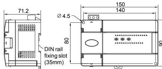
Figure 6-3 Cutout sizes of IVC1-1614MAR, IVC1-1614MAT, IVC1-1614MDR and IVC1-1614MDT
