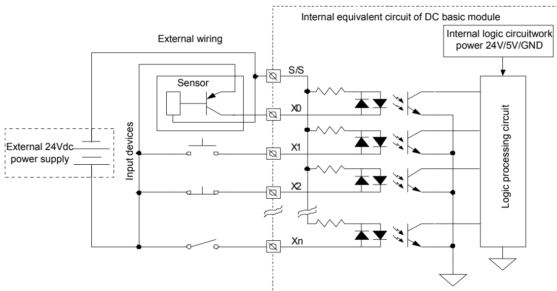
Figure 4-13 Sink input mode internal equivalent circuit of DC basic module
