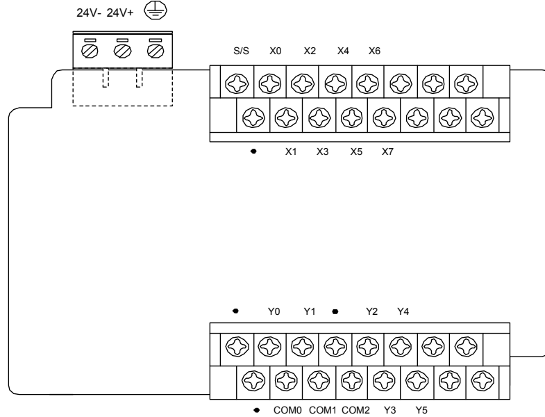
Figure 4-7 Terminals of IVC1-1006MDR and IVC1-1006MDT
