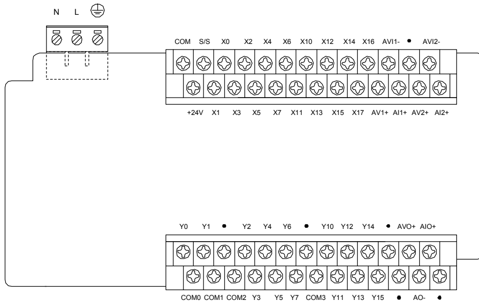
Figure 4-6 Terminals of IVC1-1614MAR1 and IVC1-1614MAT1
