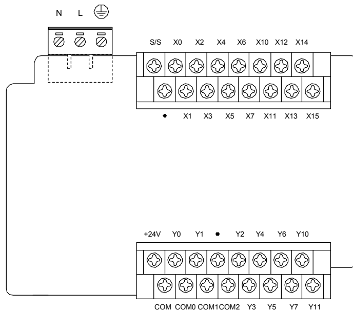
Figure 4-2 Terminals of IVC1-1410MAR and IVC1-1410MAT
