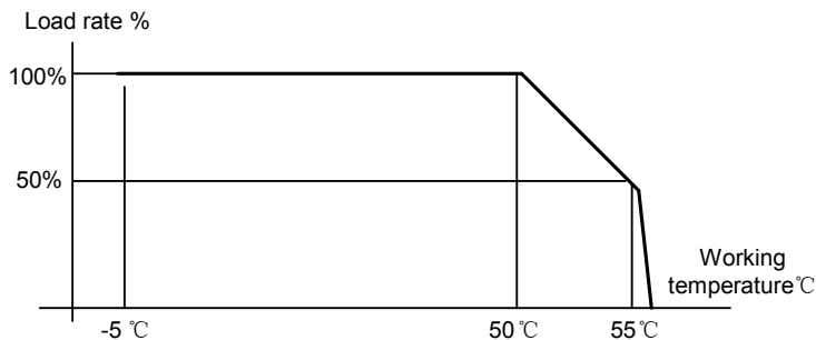
Figure 3-1 Load rate vs. working temperature
