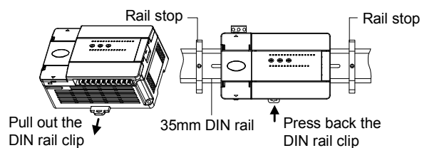
Figure 6-8 DIN rail installation
