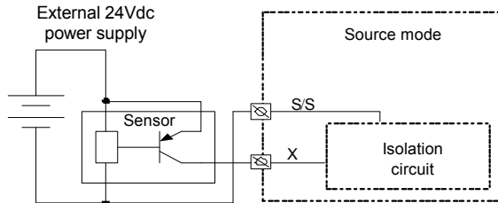
Figure 4-21 Wiring of source input mode for DC basic module
